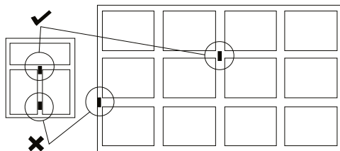
Fig. 1 Location of the detector
