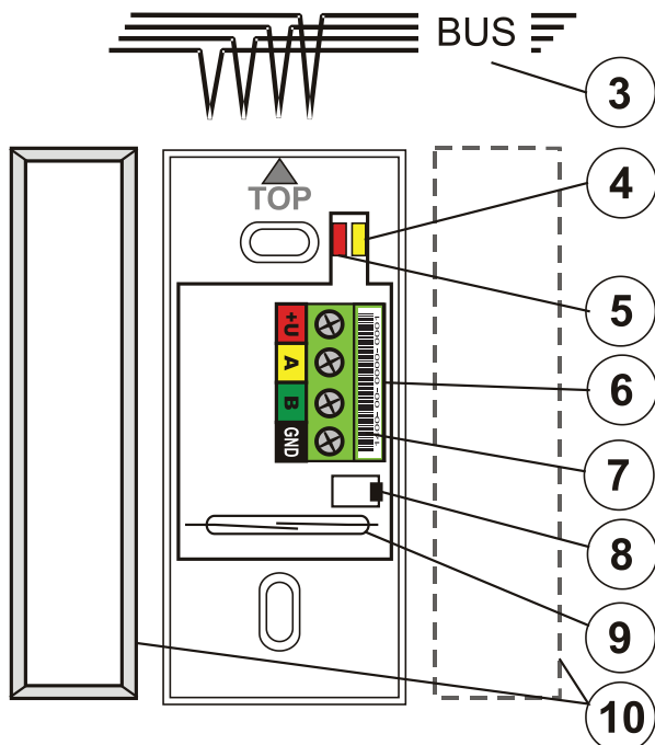
Fig: 3 – bus cable; 4 – yellow fault indicator; 5 – red detector activation indicator; 6 – digital bus terminals; 7 – production code; 8 – tamper contact; 9 – magnetic sensor; 10 – permanent magnet with its alternative position
